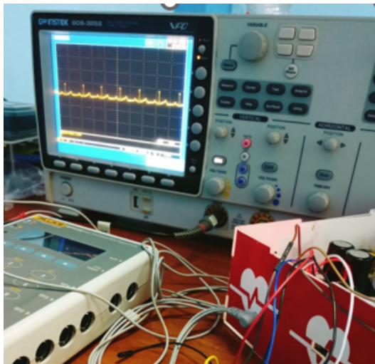
FIGURE 4. Desain ECG Instrumentation
